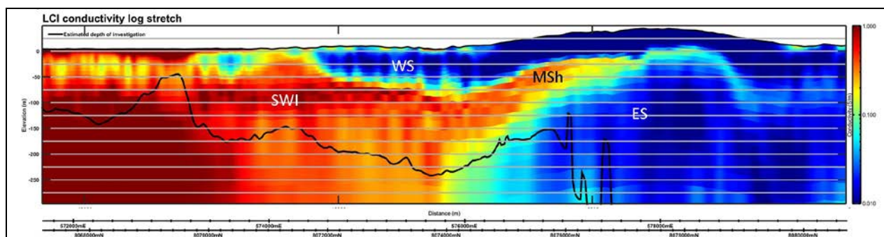
Figure 2. Conductivity depth section showing the SWI wedge, and inter-layered Wallal Sandstone, Munkyarra Shale and Erskine Sandstone.
