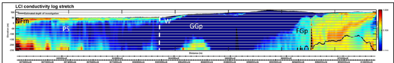
Figure 4. Conductivity depth section parallel to the May River showing the Poole Sandstone and Grant Group sandstones sub-cropping in the river bed. This reach of the river is an area of both potential recharge and groundwater discharge. The unit underlying the Grant Group is the Fairfield Group. Faulting is also evident in this section.
