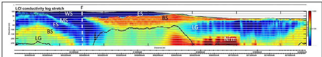
Figure 3. Conductivity depth section showing inter-layered Wallal Sandstone, Munkyarra Shale, Erskine Sandstone, Blina Shale, Liveringina Group, and Noonkanbah Formation. A significant Neogene fault is also mapped.
