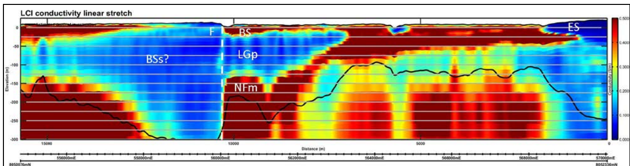
Figure 7. Conductivity depth section at a high angle to the Fitzroy River, near the river mouth. The image shows a significant Neogene fault that separates inter-layered Blina Shale, Liveringa Group and Noonkanbah Formation on the right hand side of the fault, from what is presumed to be Broome Sandstone on the left of the fault. The sharp contact along the fault between saline Noonkanbah Formation and Broome Sandstone suggests this fault may locally be a barrier to lateral groundwater flow.
